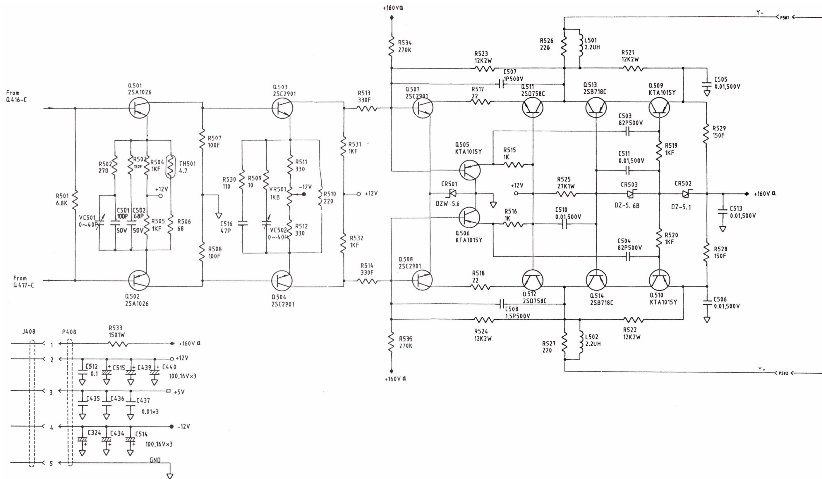
VERTICAL MAIN AMP(5)
